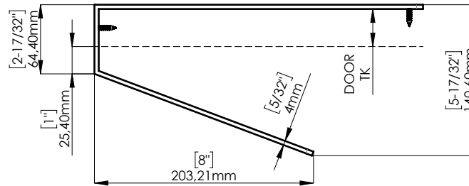
TOP VIEW SCALE 1:5
